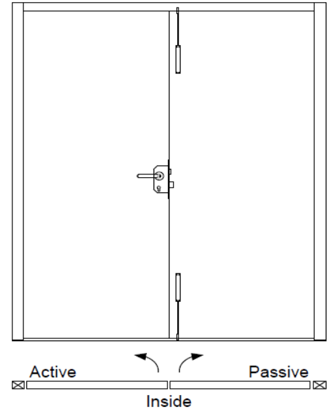
Door Hinged Left Hand Active Outward Opening - View from INSIDE
