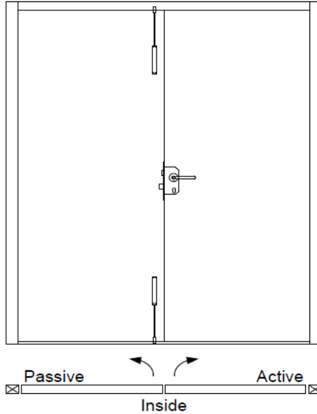
Door Hinged Right Hand Active Outward Opening - View from INSIDE
